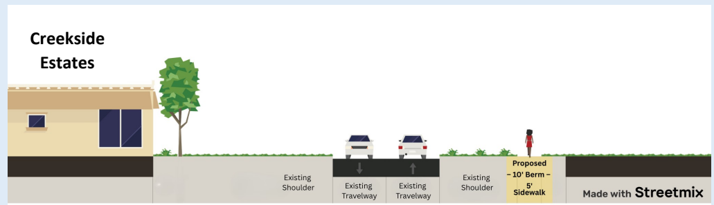
Typical Section 2 , north of the crosswalk at Chum Road, facing north.
